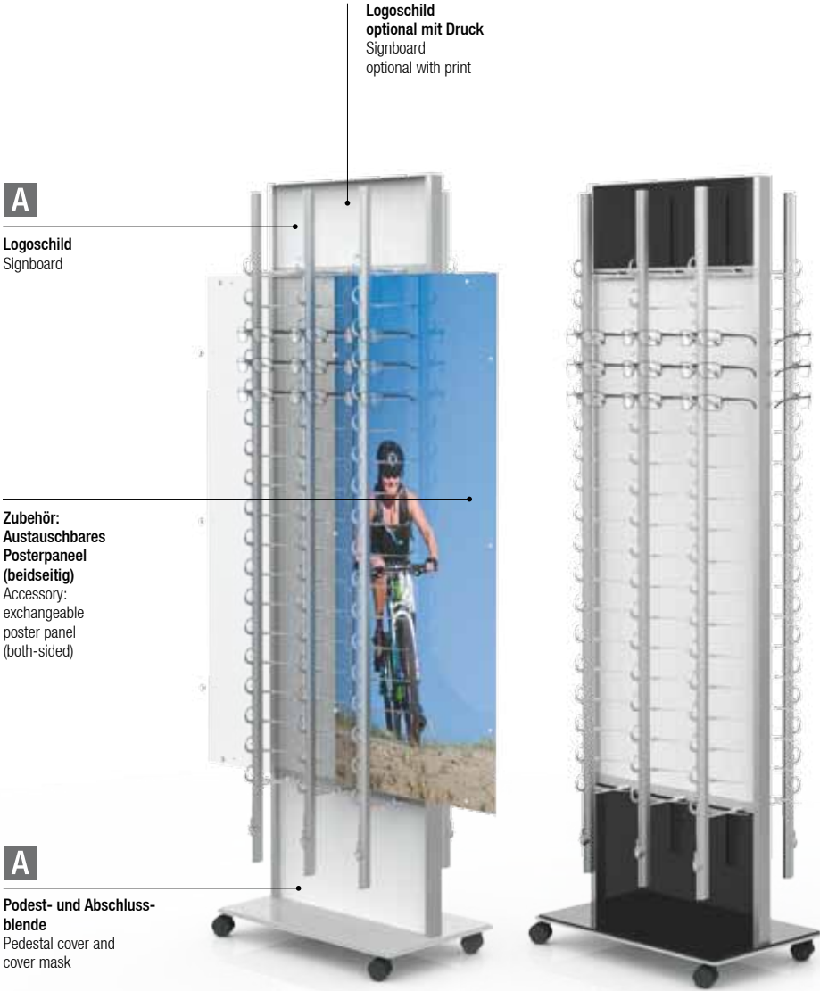
A 01 PGM 6 650 x 1925 x 400 mm 108
